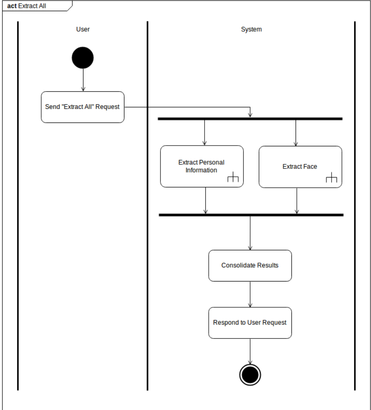
Figure 13: Extract All Activity Diagram
