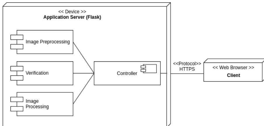
Figure 1: Deployment Diagram of Hutts Verification
